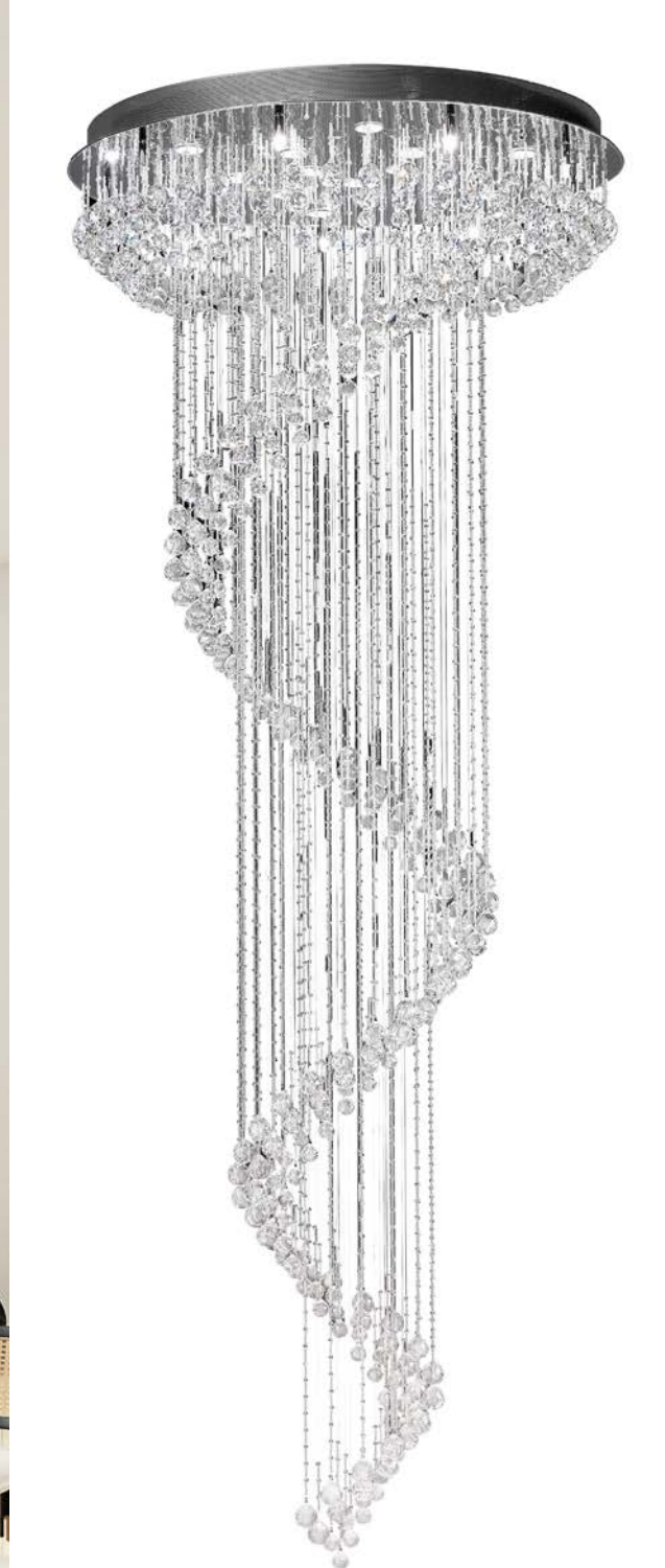
IL31376 Colorado Crystal Pendant 24 Light Ø 1000 ↓ 2550 (mm) 15 x GU10 50W, 9 x G933W, 33.8kg Polished Chrome
